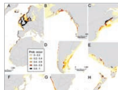
Probable range expansion for the European green crab ( C. maenas ): (a) northwestern Europe, (b) western North America, (c) eastern North America, (d) Patagonia, (e) southeastern Australia, (f) Japan, (g) South Africa and (h) New Zealand. High probabilities of occurrence are indicated by dark shading. Predictions are constrained to depths of 200m or less (as included in Compton et al. 2010).
